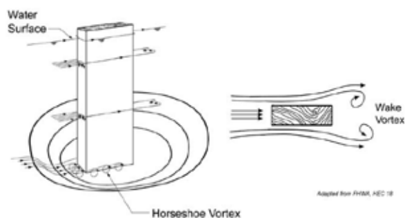
STREAM CURRENT AND SCOUR AROUND A MID-CHANNEL PIER
