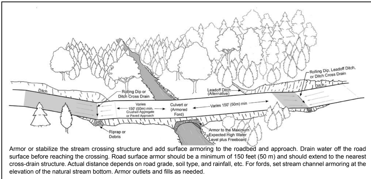
Figure 26—A sketch of a number of sediment protection measures used at a road-stream crossing, including discharging leadoff ditches into a vegetated area before reaching the stream.
