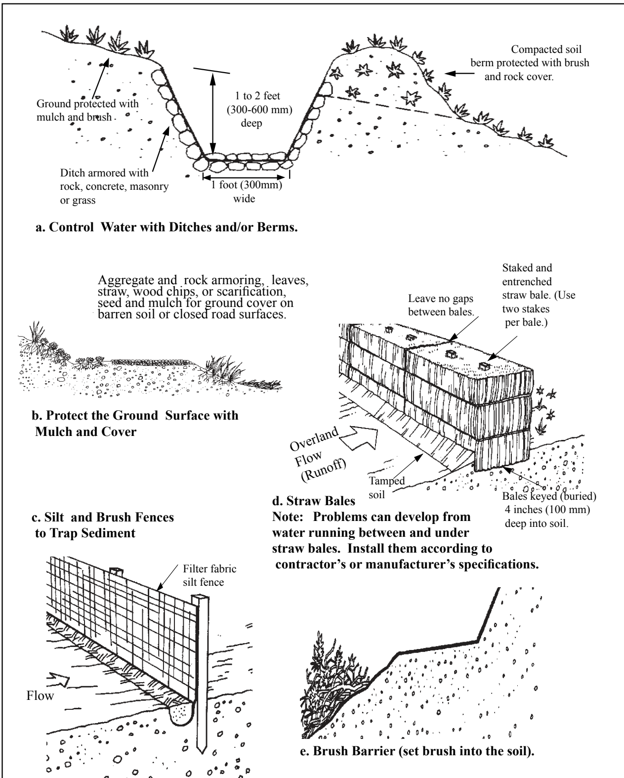
Figure 47—Common physical erosion control measures.
