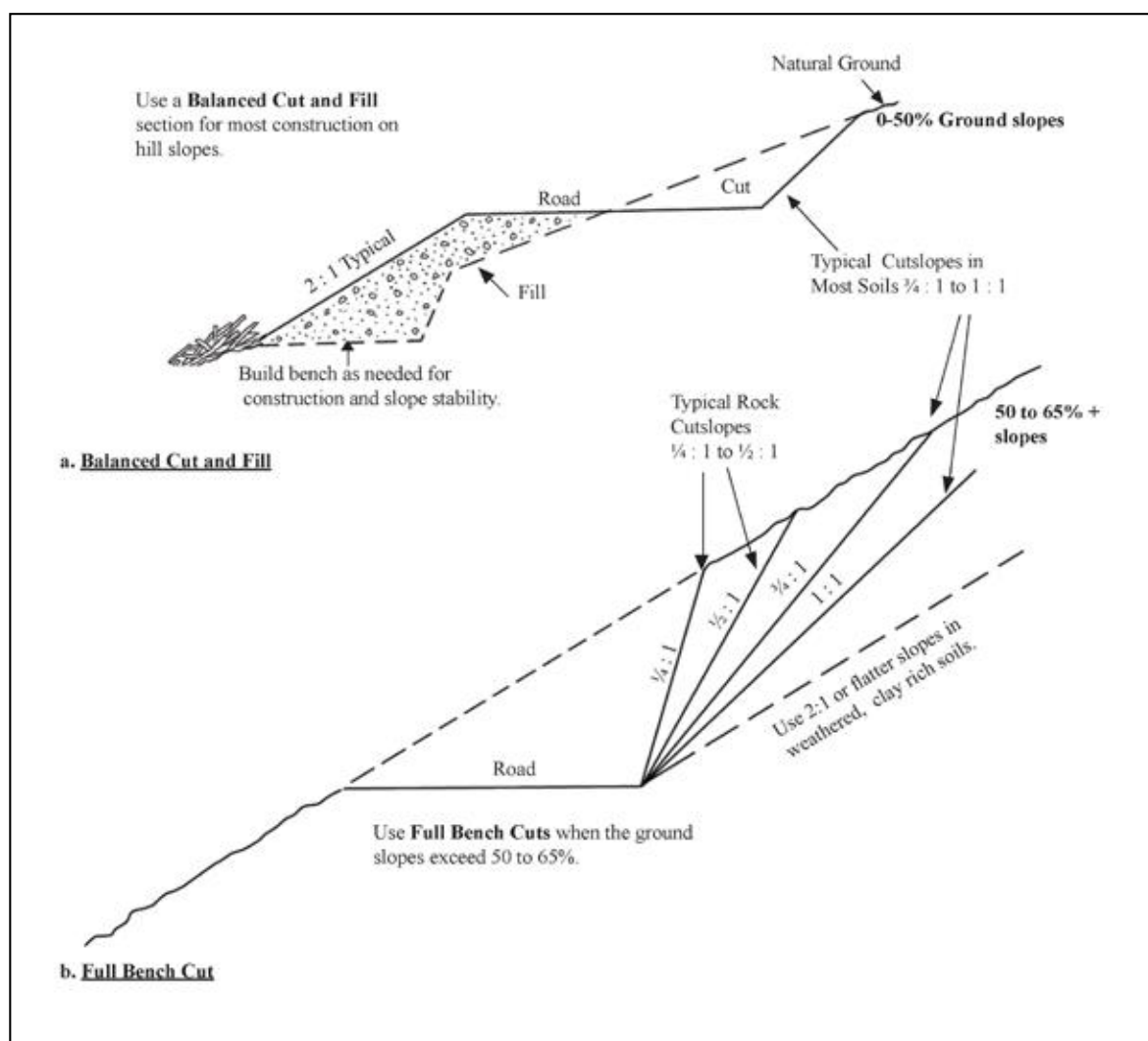
Figure 129—Commonly used stable cutslope angles.
