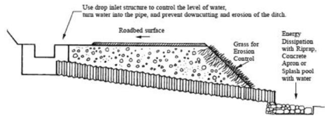
FIGURE 12 Typical drop inlet structure with culvert cross-drain (Keller and Sherar 2003).
