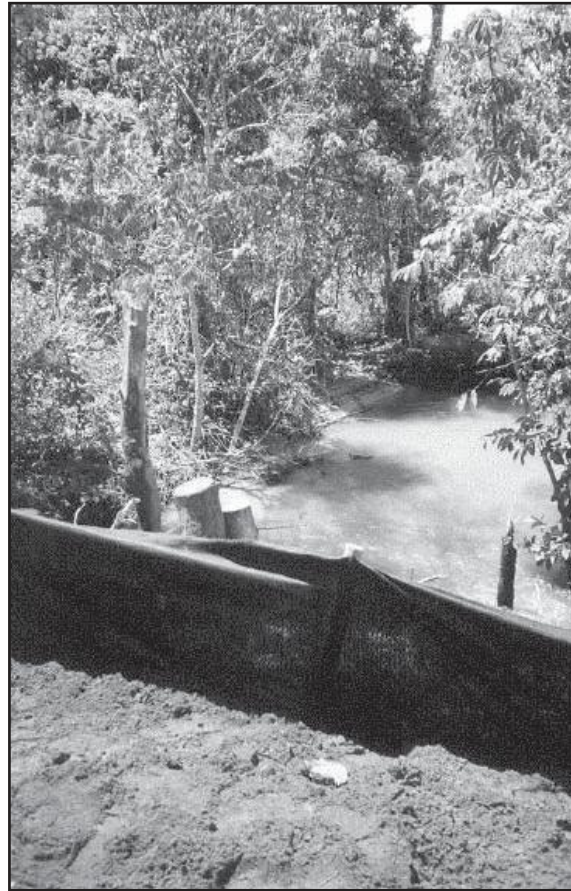
Sheet piling in conventional river crossings
